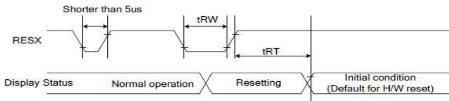
Figure 126: Reset Timing
