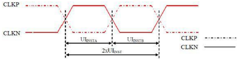
Figure 118: DSI Clock Channel Timing
