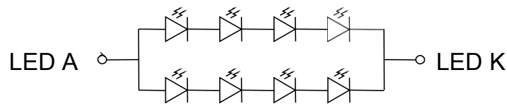
LED CIRCUIT
